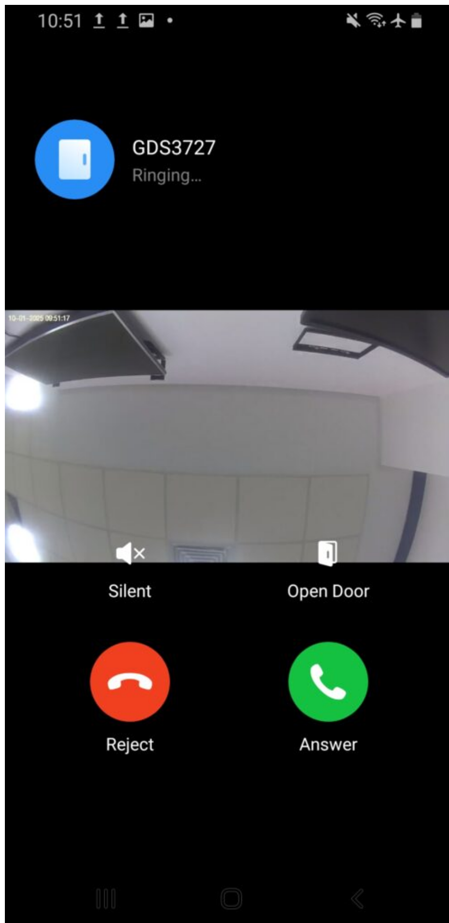
Incoming Call
