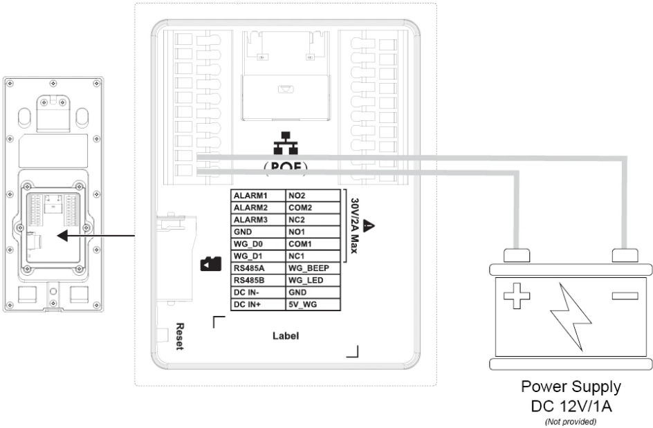
Powering the GDS3726 using a Power Supply
