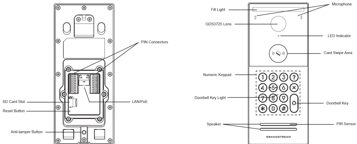
GDS3725 Front and Back View
