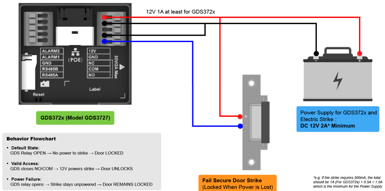
GDS3727 with Fail Secure Door Strike
