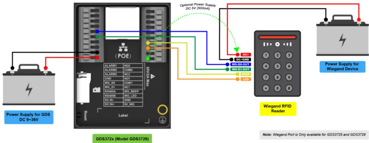
GDS372x with Wiegand RFID Reader
