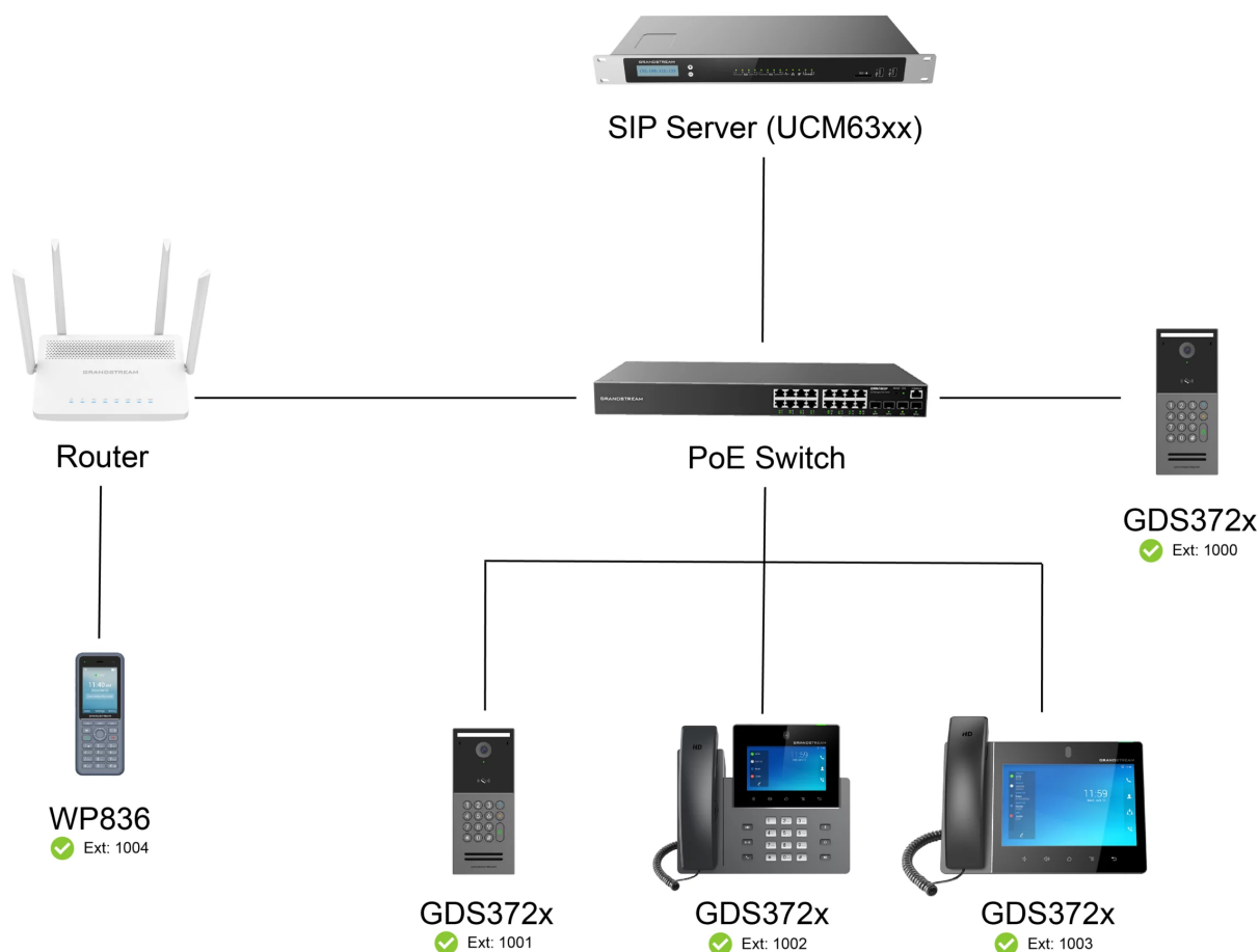
Peering GDS372x with SIP Server
