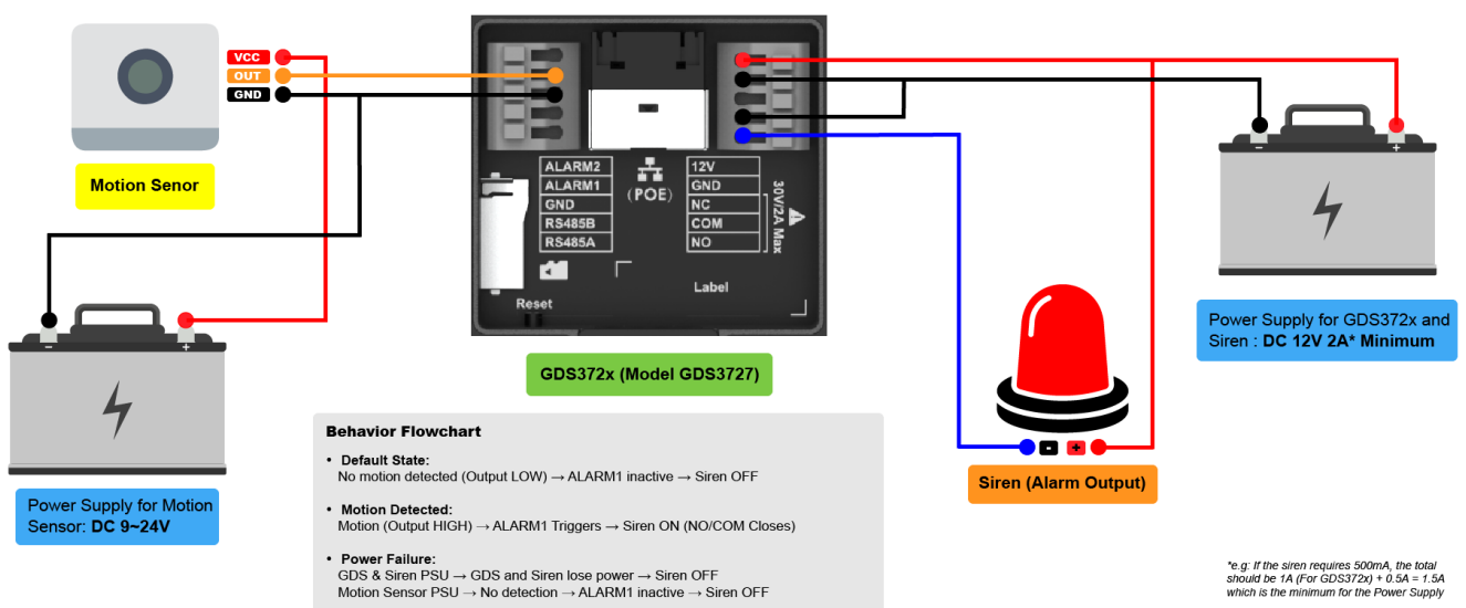
GDS372x with Siren and Motion Sensor
