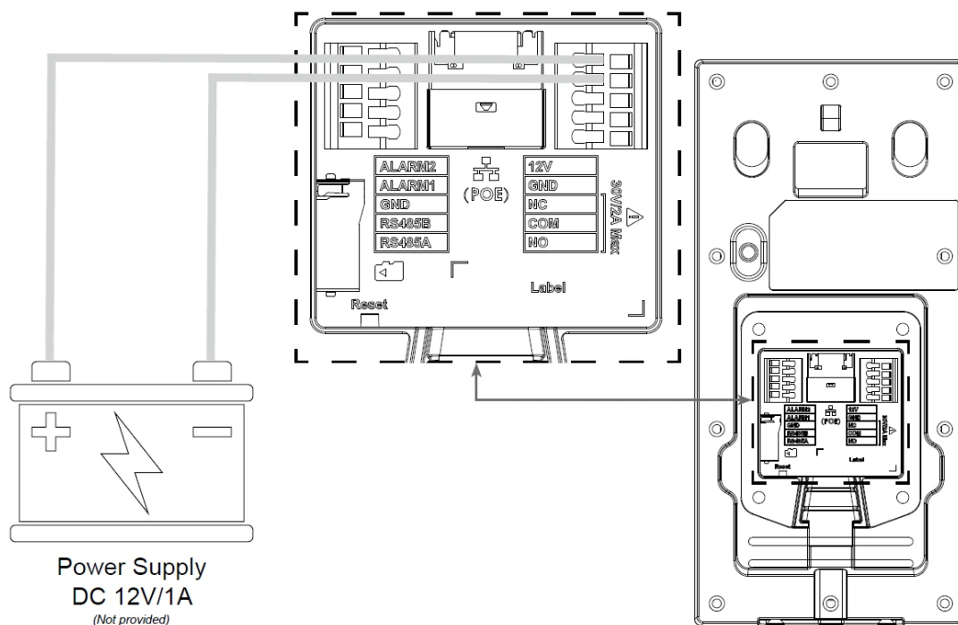
Powering the GDS3727 using a Power Supply
