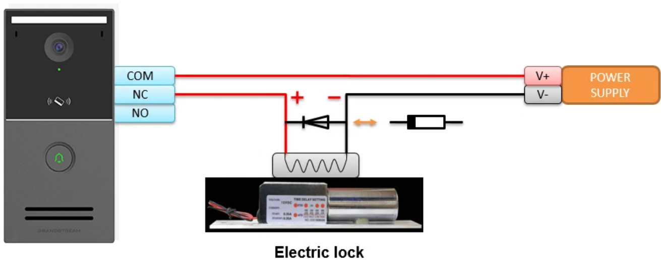
Protection Diode Example 1
