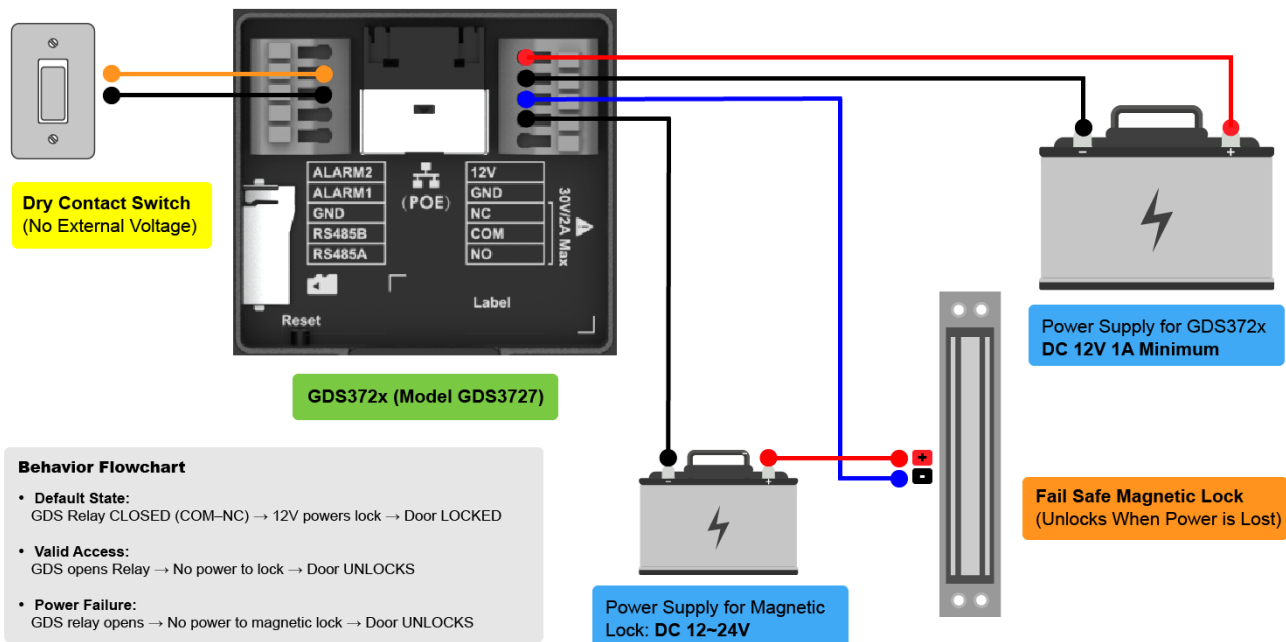
GDS372x with Fail Safe Magnetic Lock and Dry Contact Switch
