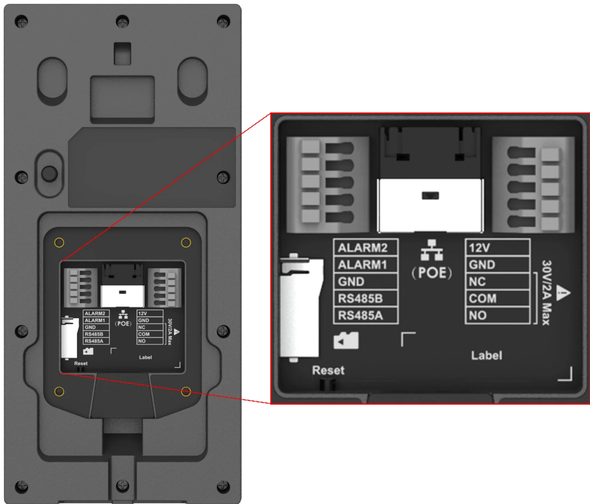
GDS3727 Wiring Connection
