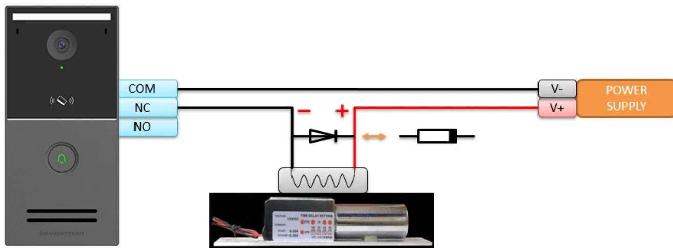
Electric lock
