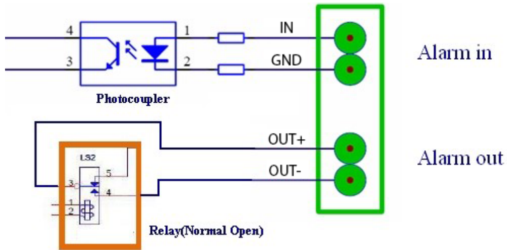
Alarm InOut Circuit for GDS372x
