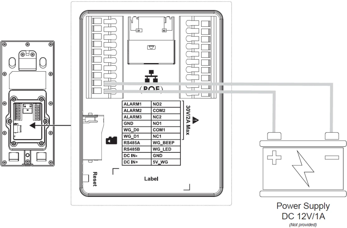
Powering the GDS3725 using a Power Supply
