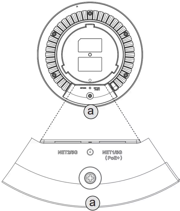
GWN7672 Ports
