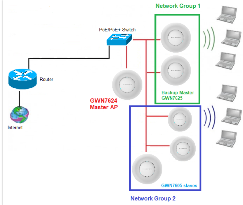
Failover Master
