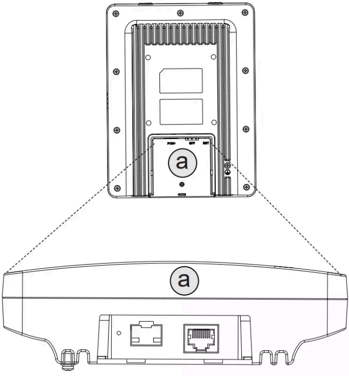
GWN7670LR Ports
