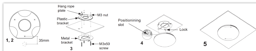
Ceiling Mount
