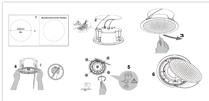
Ceiling Mount
