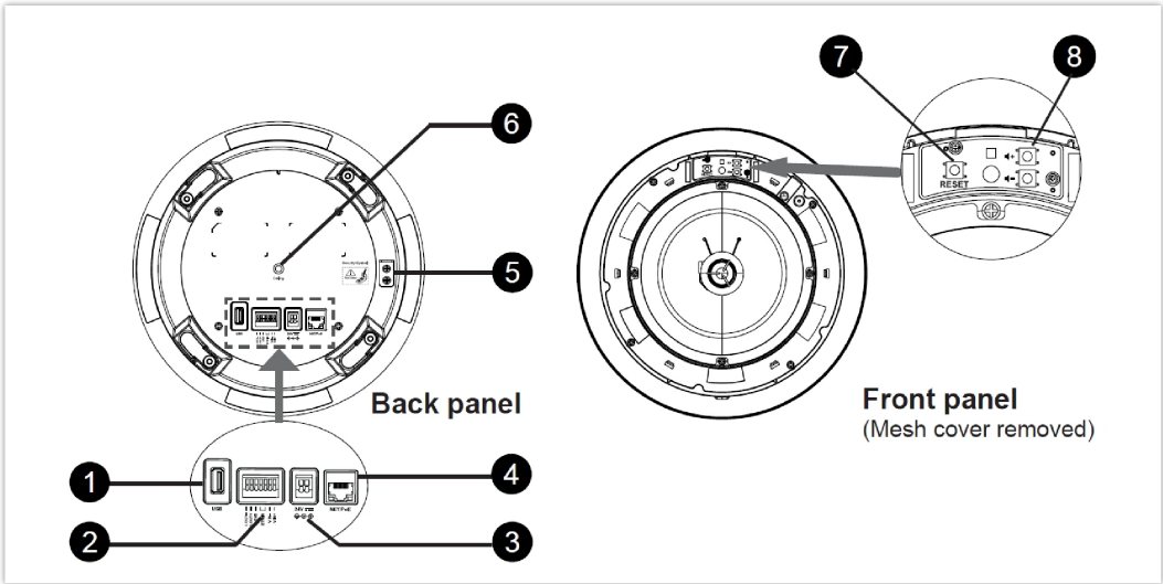
GSC3506 V2 Ports and Buttons
