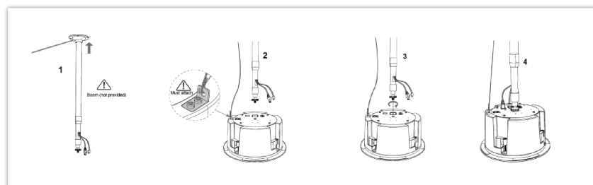
Boom Mount
