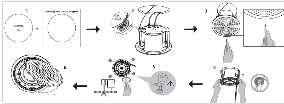
GSC3506 V2 Ceiling Mount
