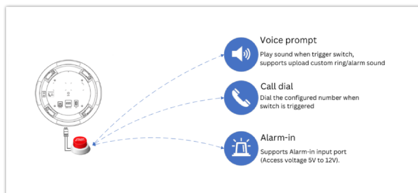
2 pin Multi Purpose Input Applications for GSC3506 V2
