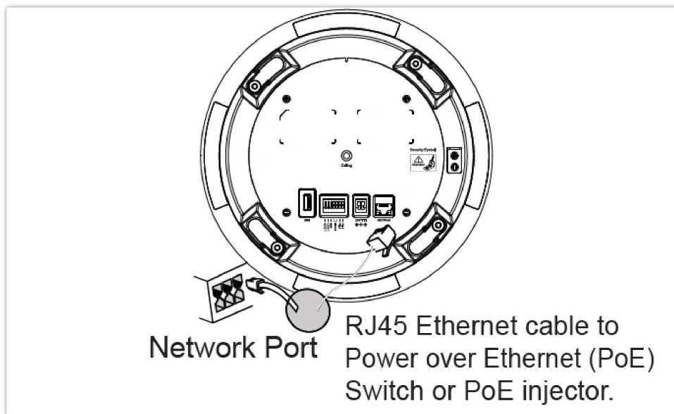
Powering GSC3506 V2 using PoE
