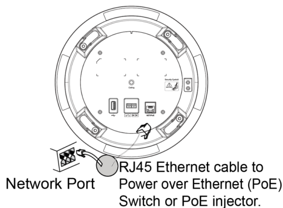
Powering GSC3506
