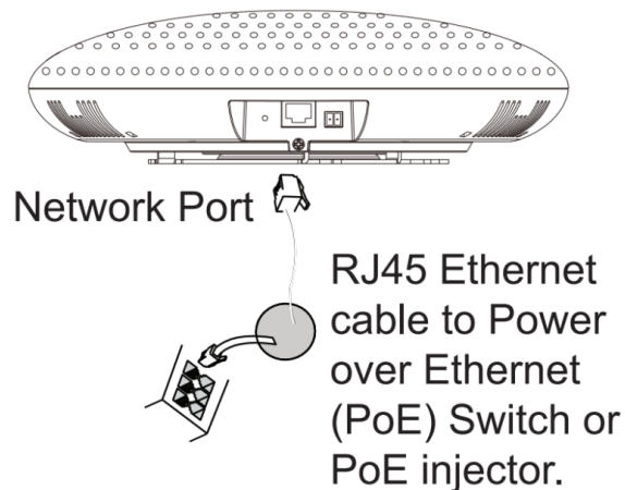
Powering GSC3516
