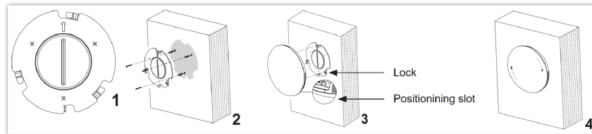
Wall Mount
