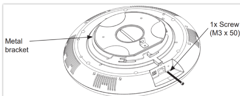
Anti theft Installation
