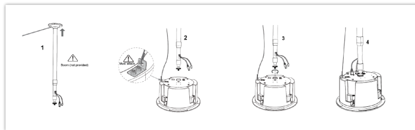
GSC3506 V2 Boom Mount
