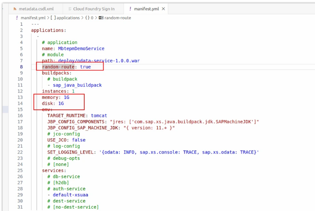
manifest.yml
